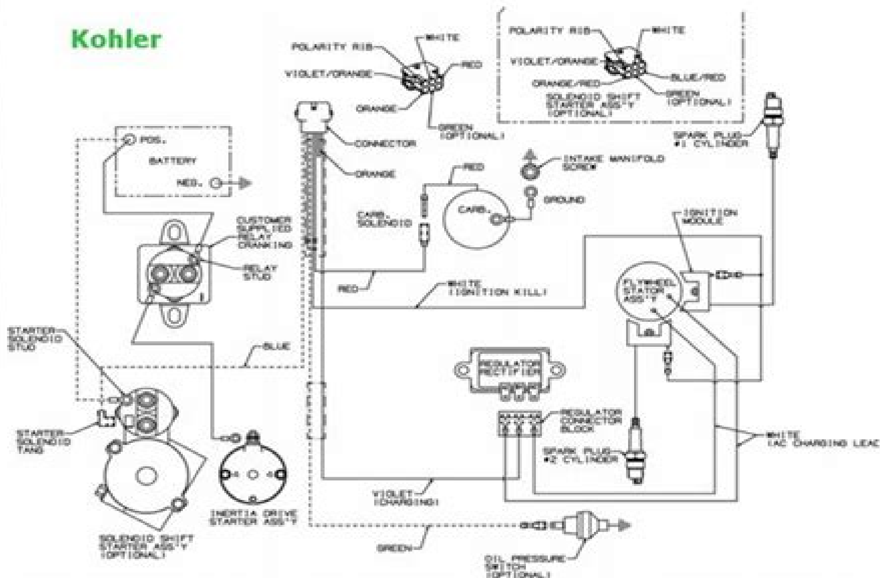
Figure 7-16. Wiring Diagram - Fixed Timing Ignition System.
