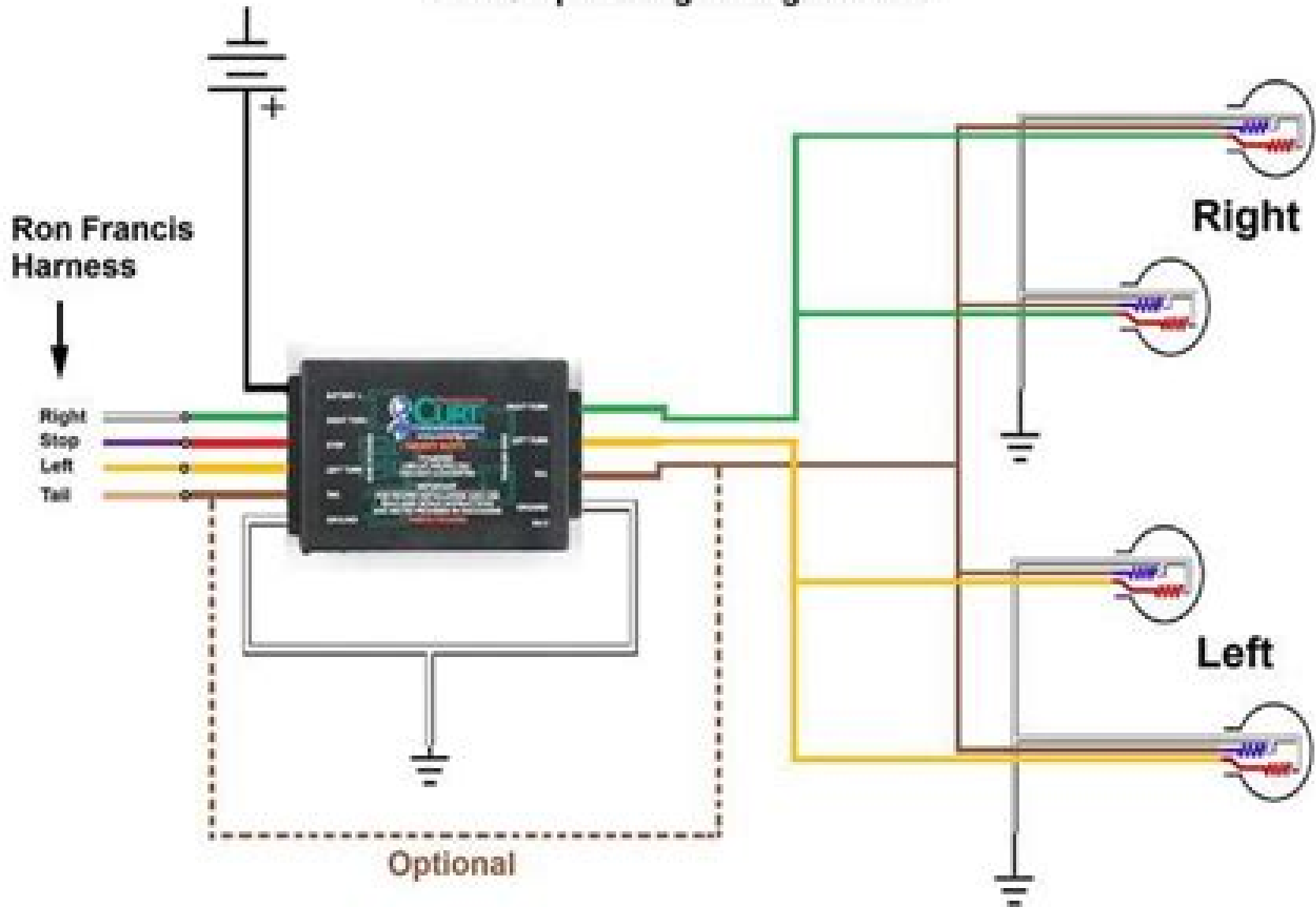
Turn-Stop-Tail Light Diagram - 1.1
