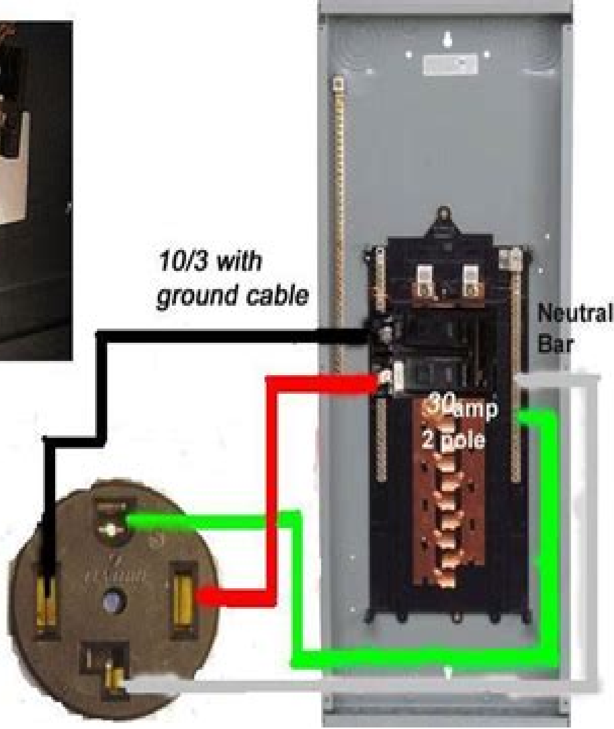
Dryer Connections
