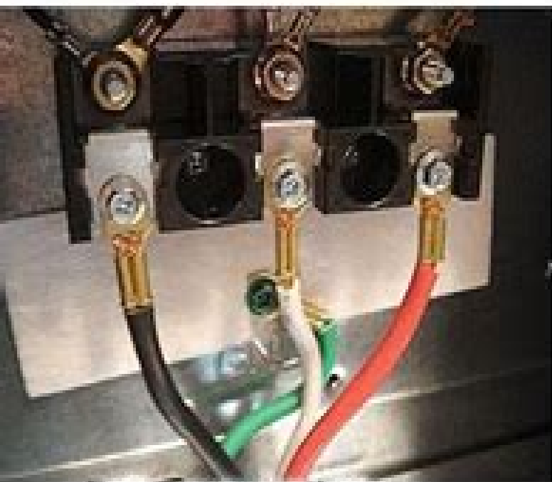
Dryer Connections
