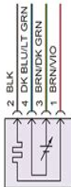
OXYGEN SENSOR 2/1
