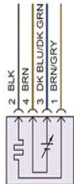
OXYGEN SENSOR 2/2 (RIGHT SIDE OF TRANSMISSION)
