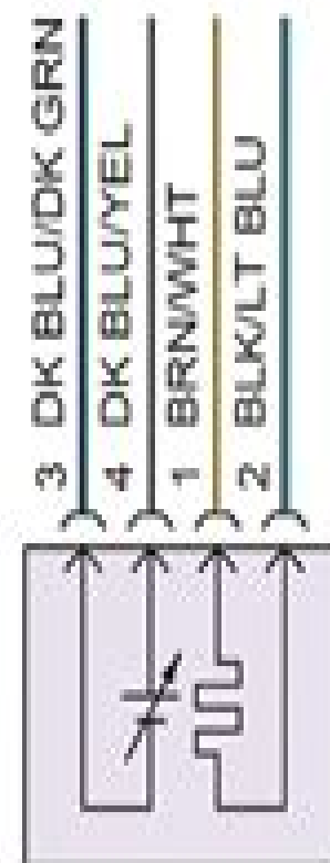
OXYGEN SENSOR 1/2 (AT: BELOW TRANSMISSION, IN LEFT EXHAUST PIPE)
