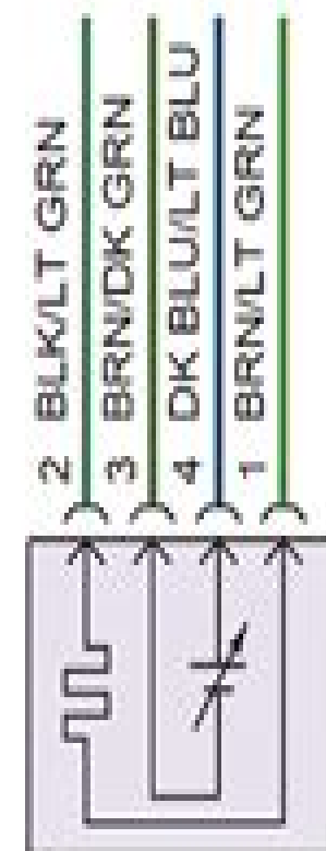
OXYGEN SENSOR 1/1 (M/T: BELOW RIGHT FRONT OF TRANSMISSION, IN EXHAUST) (AT: LEFT SIDE OF TRANSMISSION)
