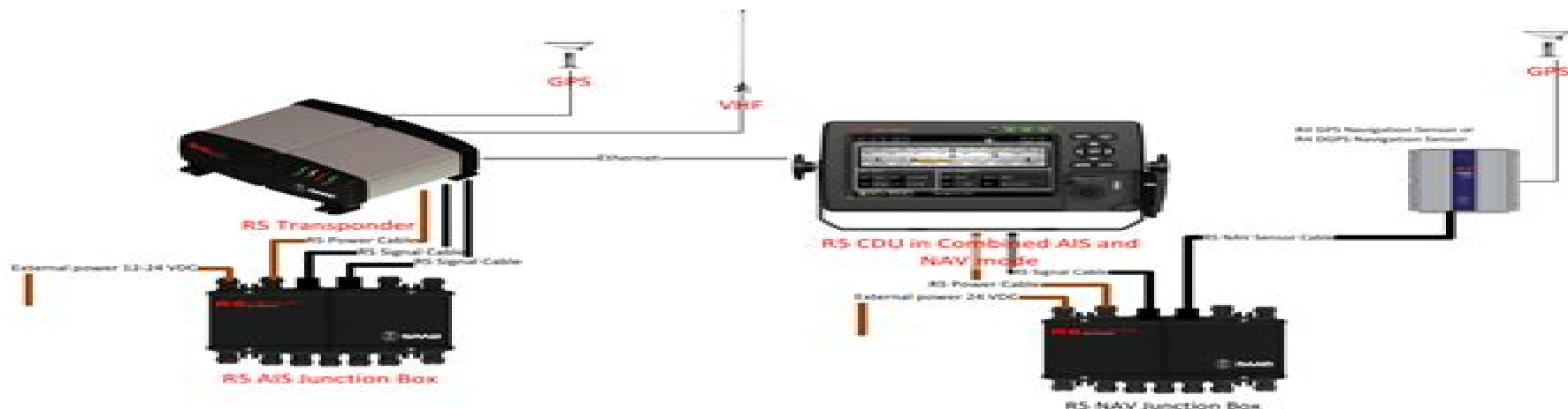
Figure 46- Combined AIS and Navigation system
