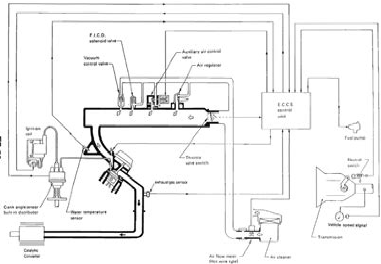
E.C.C.S. DIAGRAM
