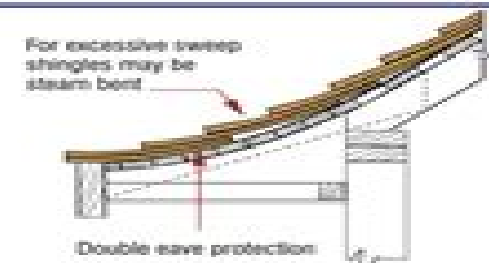
Figure 12: Swept or Bell Eave
