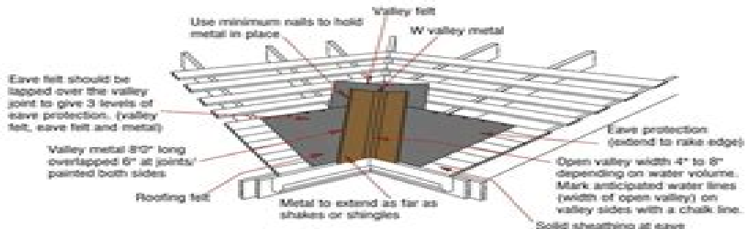
Figure 13a: Valley Metal
