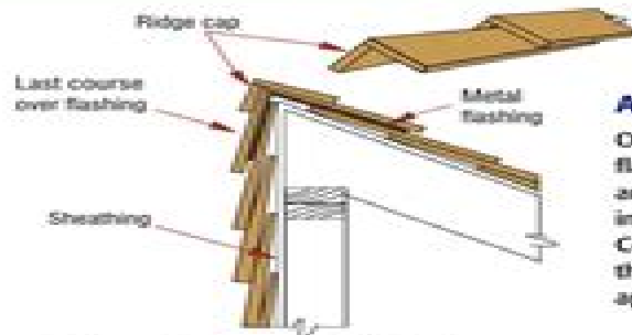
Figure 11: Apex Roof Junction
