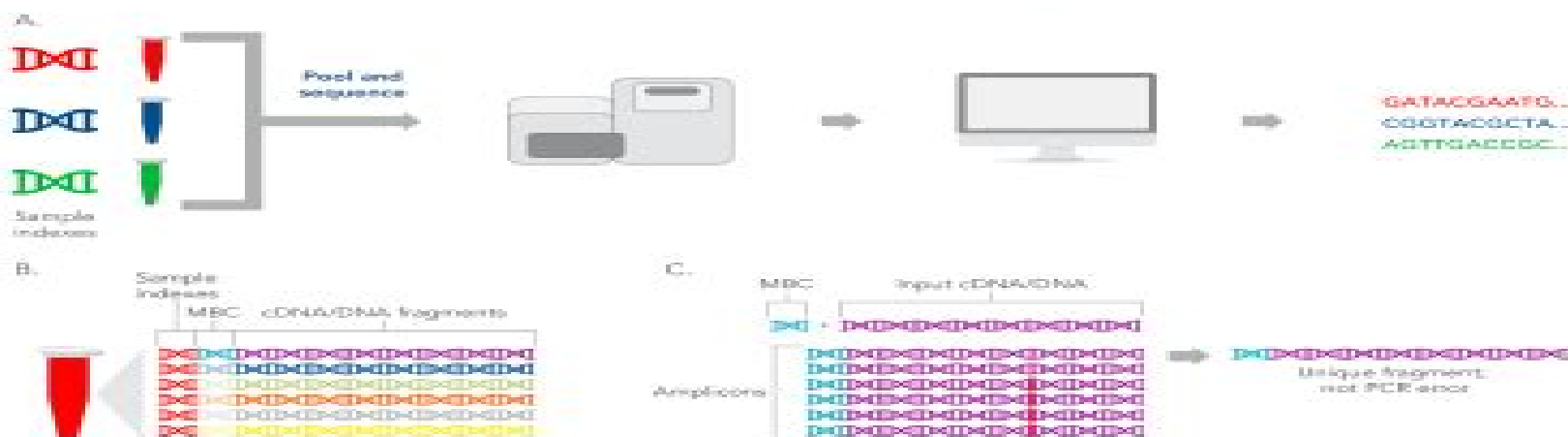
Figure 1. Sample indexes differ from molecular barcodes (MBCs). (A) Each sample is labeled with a unique sample index. The sample libraries are then sequenced, and analysis software bins the data based on the index in each sample. (B) Each cDNA or DNA molecule in a sample has the same sample index, but a unique MBC ligated before amplification. (C) After amplification and sequencing, the software generates consensus sequences based on MBCs, which helps remove PCR errors (red lines) or amplification bias.
