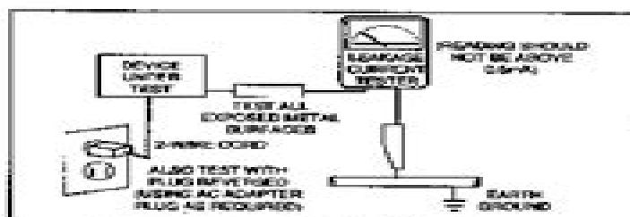
Fig. 1-1 AC Leakage Test
