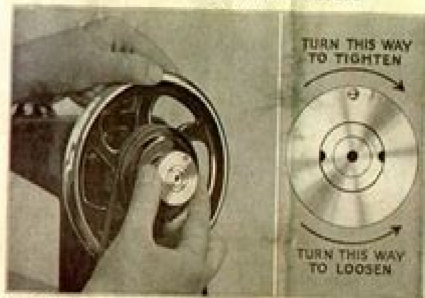
Figure 1. To release the sewing mechanism, hold the hand wheel with your left hand and turn the brake button out with your right hand. The picture on the right shows the direction to turn the brake button to tighten or loosen it. It is only necessary to turn the brake button about one half turn.
