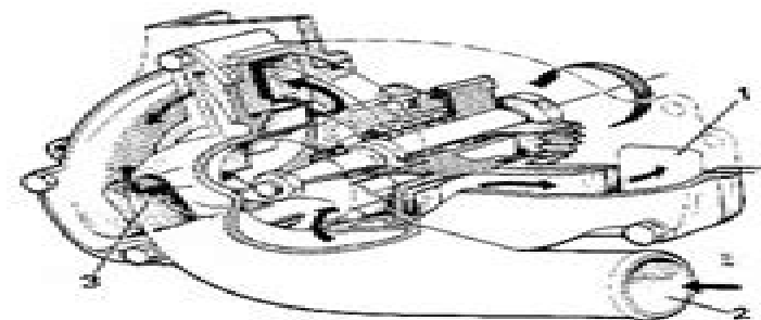
1. Outlet to engine 2. From radiator 3. Outlet to engine
