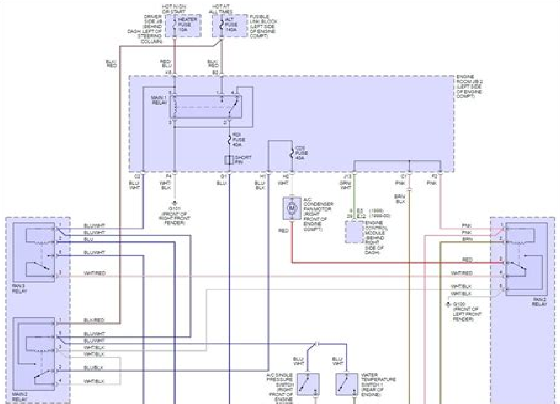
Fig 1: Cooling Fan Circuit, W/ Towing Package
