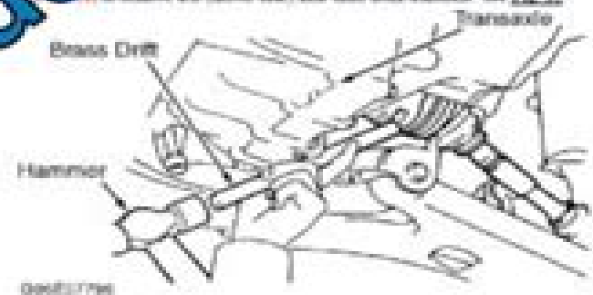
Fig. 14. Removing Right Drive Shaft (2WD Models) Courtesy of TOYOTA MOTOR SALES, U.S.A., INC.
