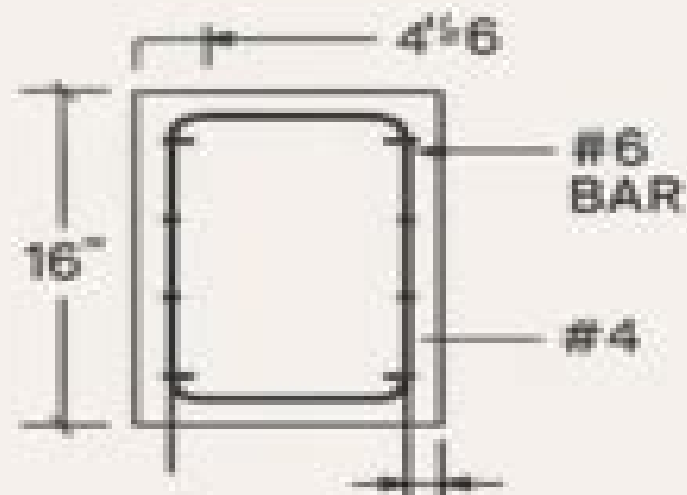
T15 - #3 TIES @ 6"
