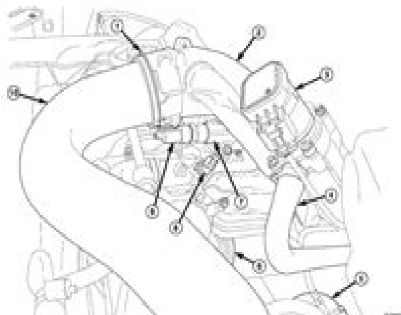
Fig. 09 INTAKE MANIFOLD
