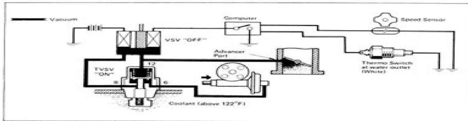
Fig. 6-4 TCS System Operation ("OFF" Condition (2))
