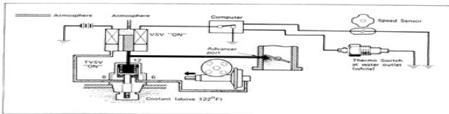
Fig. 6-5 TCS System Operation ("ON" Condition)
