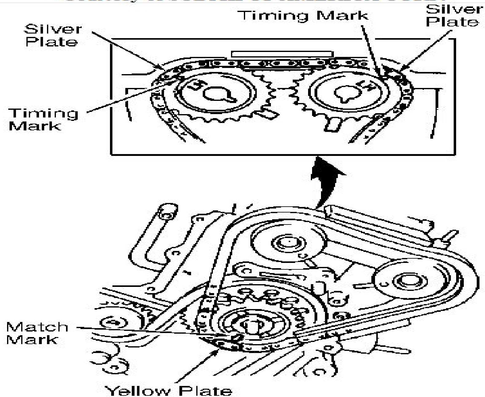
Fig. 8: Locating Left Bank Camshaft Timing Chain Marks Courtesy of SUZUKI OF AMERICA CORP.
