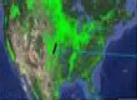
1. Cropland extent @ 30m www.croplands.org
