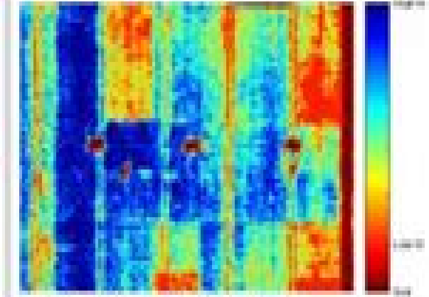
11. Nitrogen map of corn, hyperspectral data
