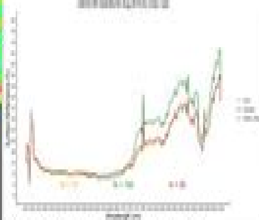
7. GLR DESIS spectral library of crops, Aug. 2010
