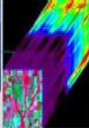
4. GLR DESIS data-cube
