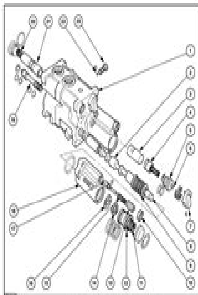
Front Wheel Hydraulic Control Valve
