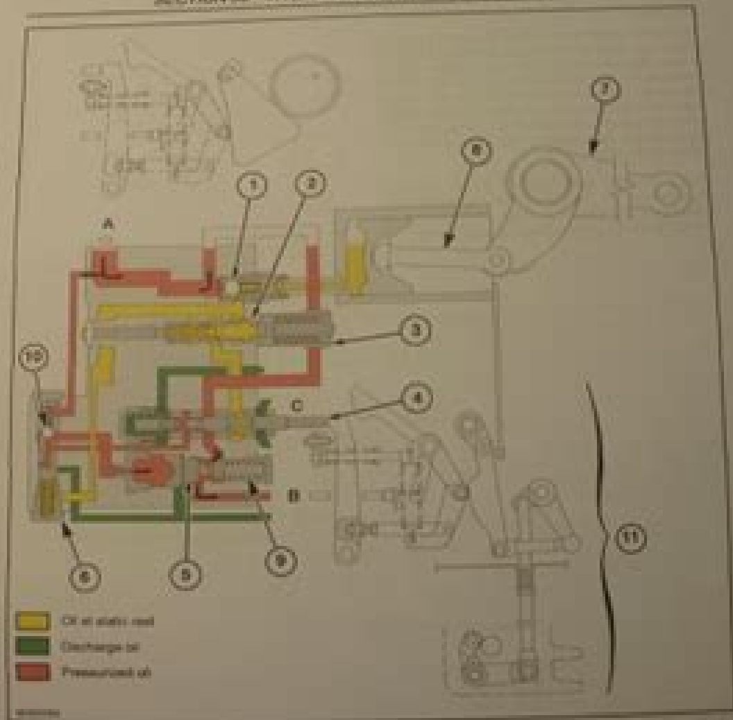
Hydraulic Power Lift (HPL) Control Valve Neutral Phase
