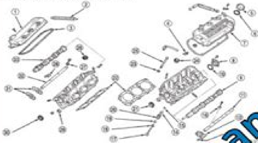
Fig. 4 Cylinder Head and Valvetrain
