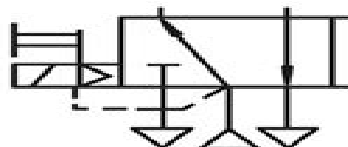
Solenoid with manual override and integral pilot
