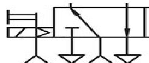
Solenoid with external pilot supply
