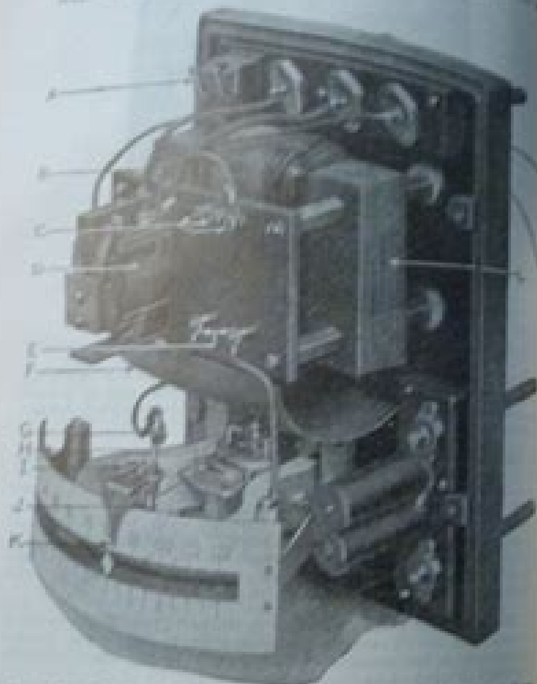
FIG. 32A.—Type TRD-A Temperature Indicating Relay: Right Front Cover Removed.
