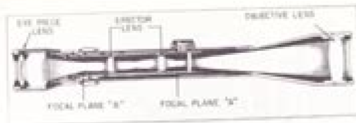
Figure 4. --Optical System.
