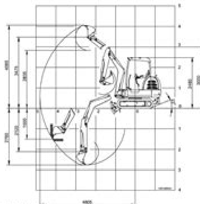
Fig. 3-Pg. 3 Working diagram
