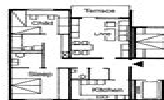
12 Accessible flat for four people in a block with three flats per floor
