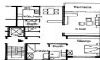
11 Accessible flat for three people in a block with two flats per floor
