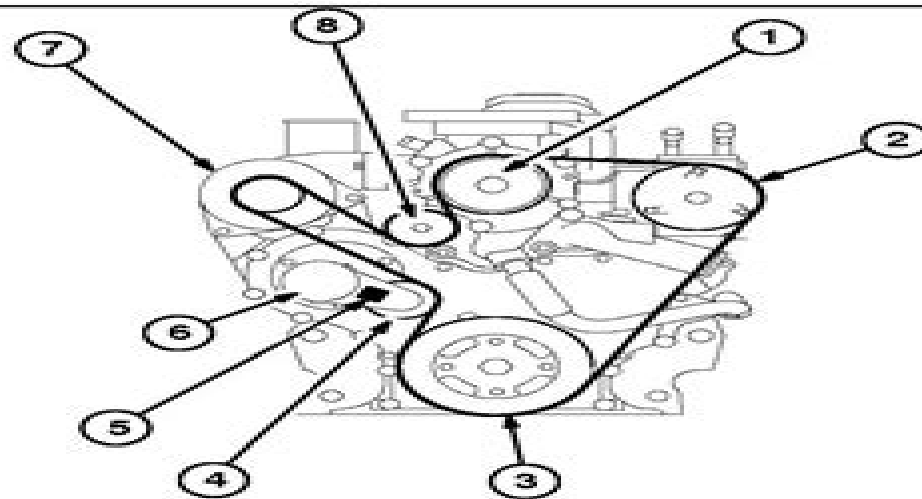
Fan Belt Tensioner
