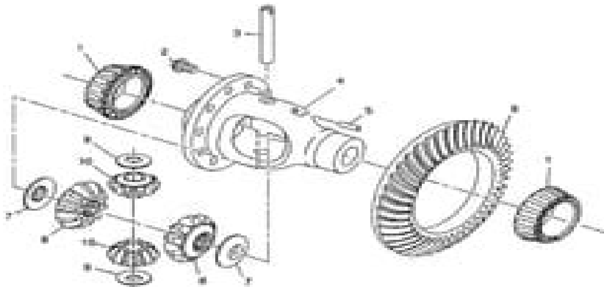
Fig. 2: Differential Carrier Components Courtesy of GENERAL MOTORS CORP.
