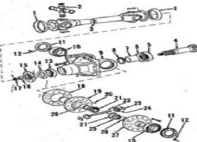
Fig. 12—Exploded view of front drive differential and drive shaft used in Model 1210 four-wheel drive truck.
