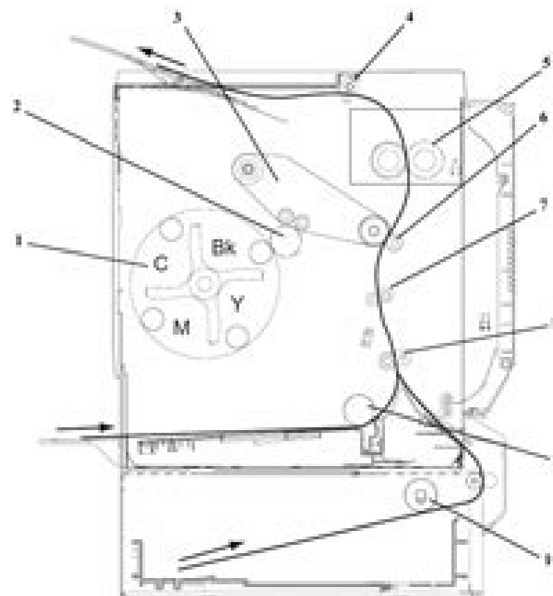
Figure 2-1. Sectional View of Mechanism
