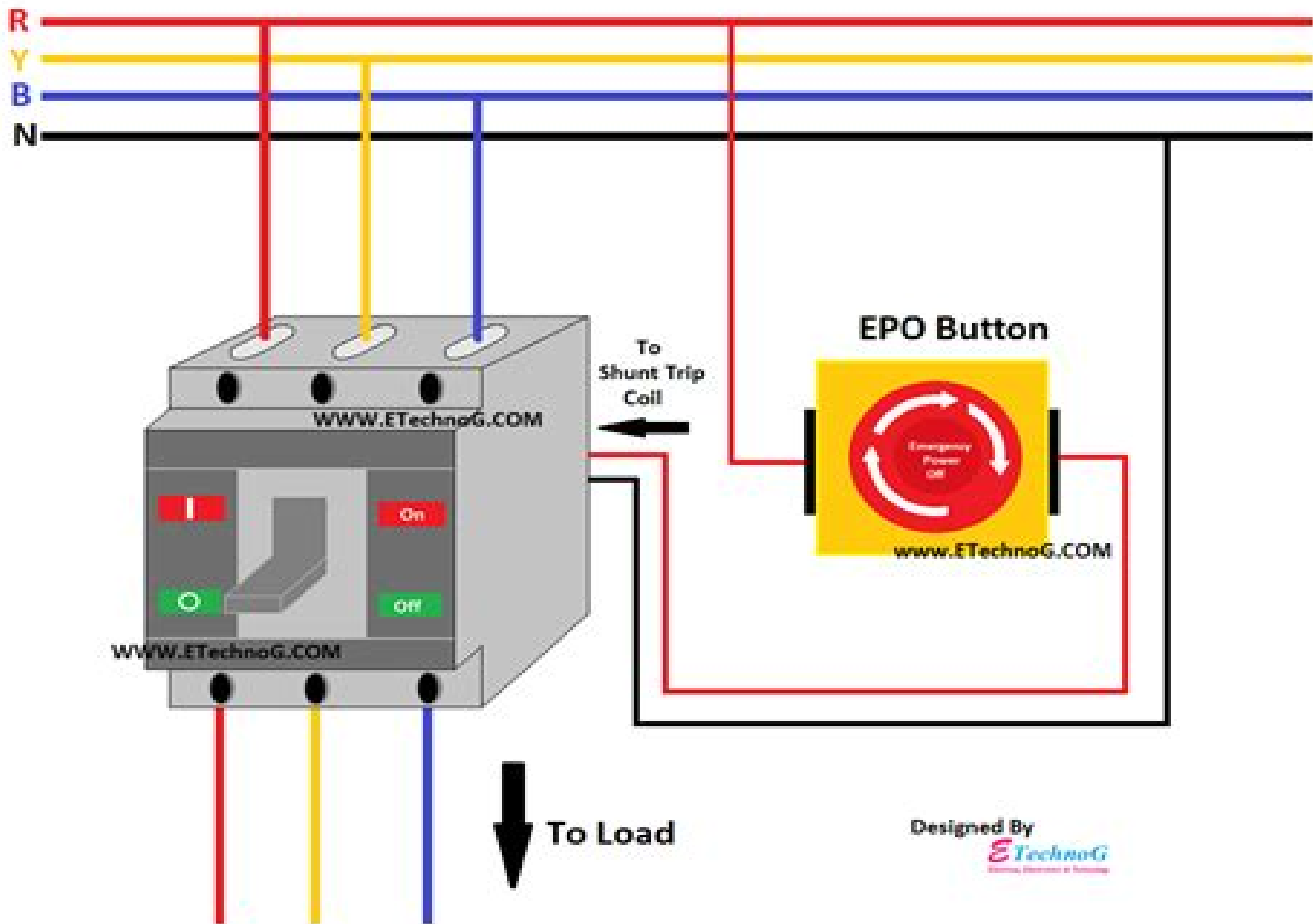
Shunt Trip Breaker Wiring Diagram and Connection
