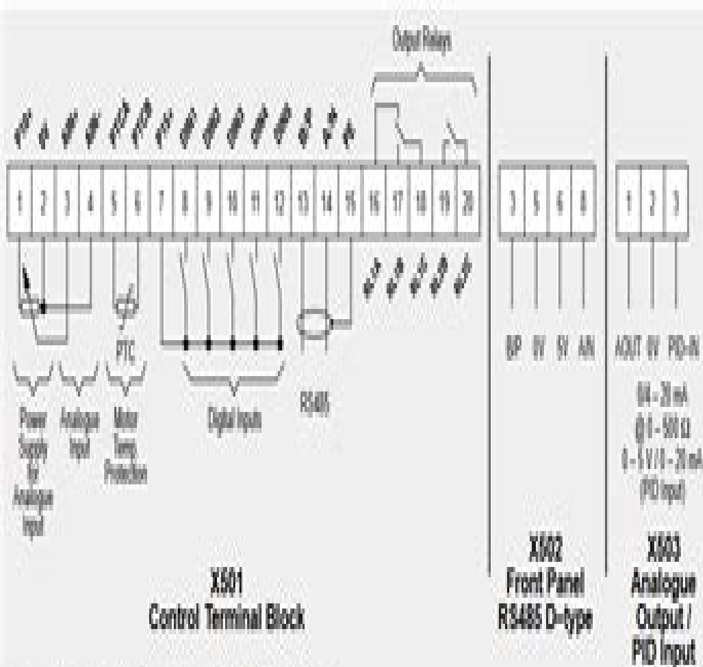
Figure 7: Control Connections - MICRO MASTER
