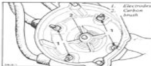
Fig. B-16 Check distributor cap and electrodes
