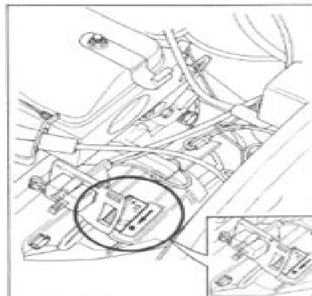
Fig. B-20 Engine type 841/A2M timing marks (auto)
