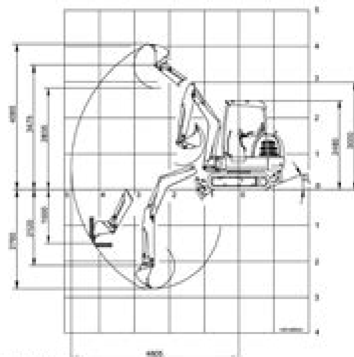
Fig. 3-Pg. 3 Working diagram
