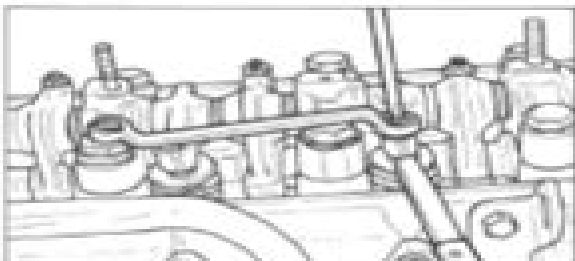
Fig. 8-7 Checking/adjusting valve clearance - OHC
