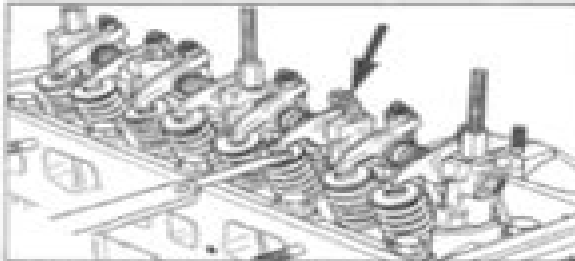
Fig. 8-5 Checking/adjusting valve clearance - OHV
