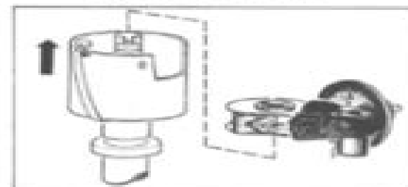
Fig. 8-10 Lifting out "cassette" type points assembly
