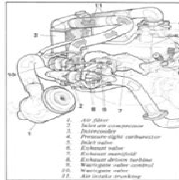
Fig. 8-6 Details of the turbocharging system - 907 type
