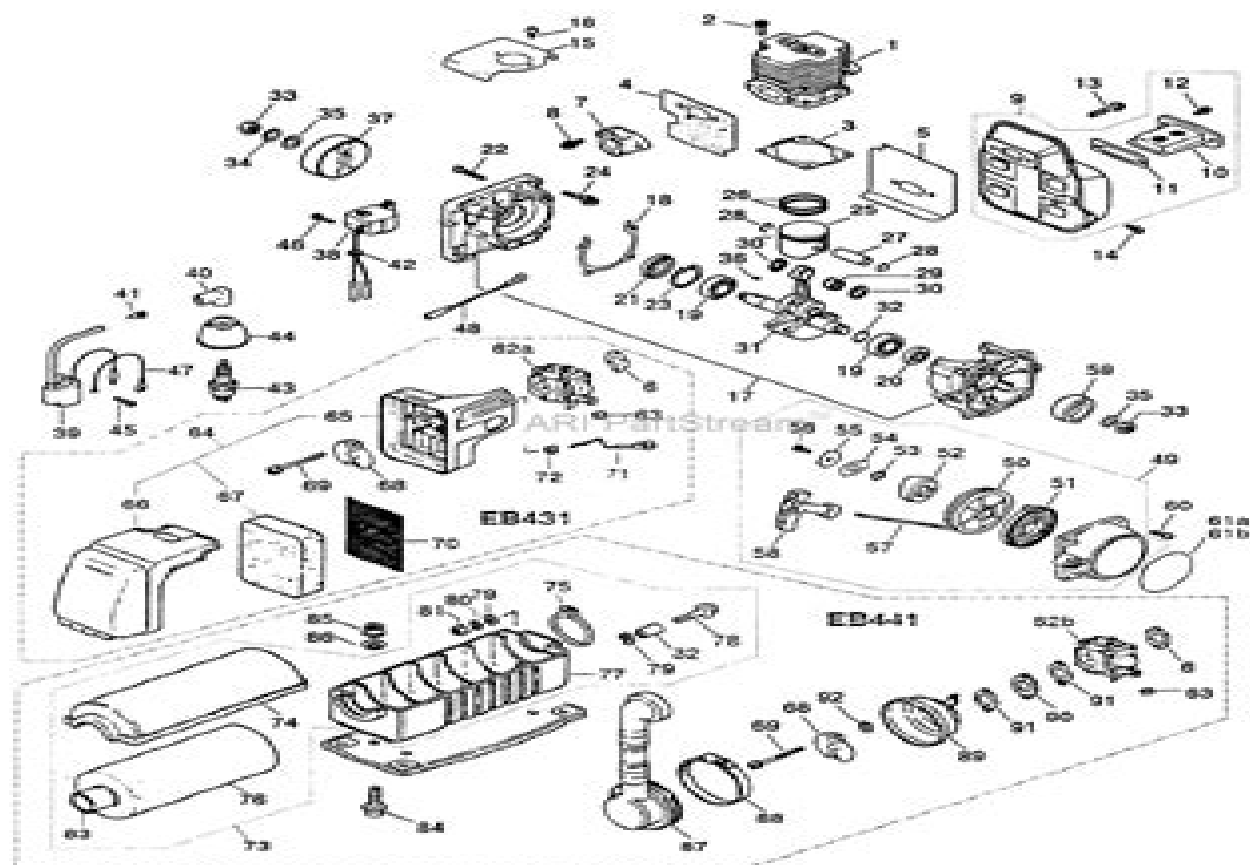
FIG. 1 ENGINE GROUP
