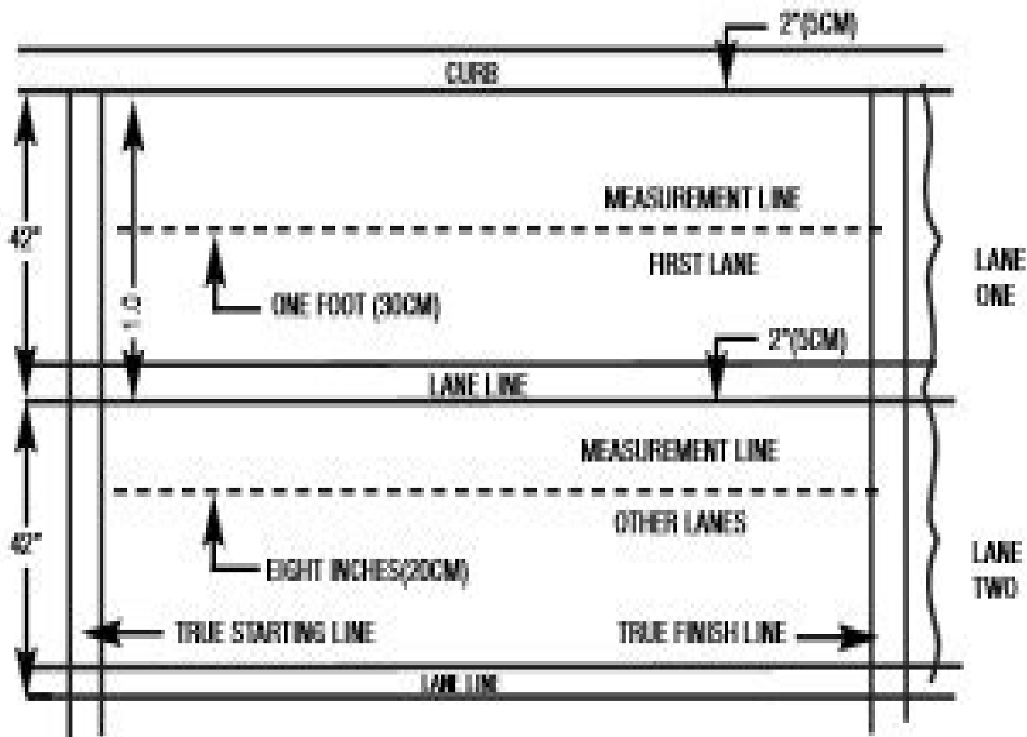
FIGURE 1 - TRACK MEASUREMENTS
