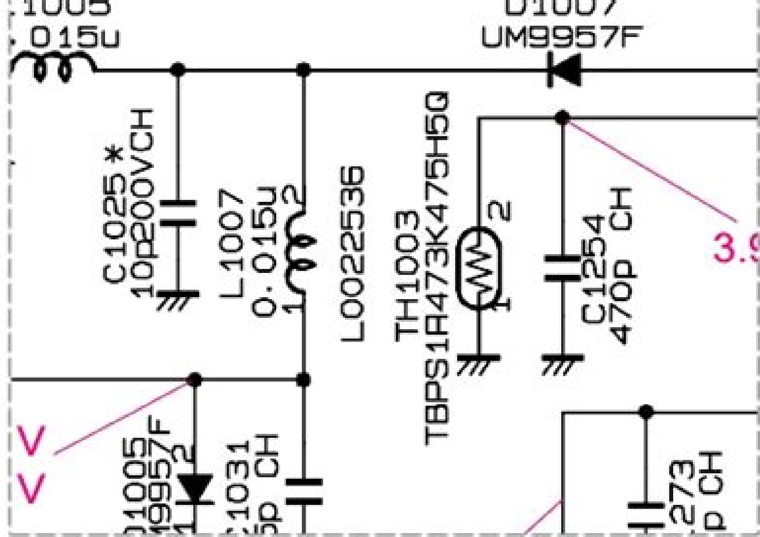
Preview: YAESU VX-2500U schematic diagram
