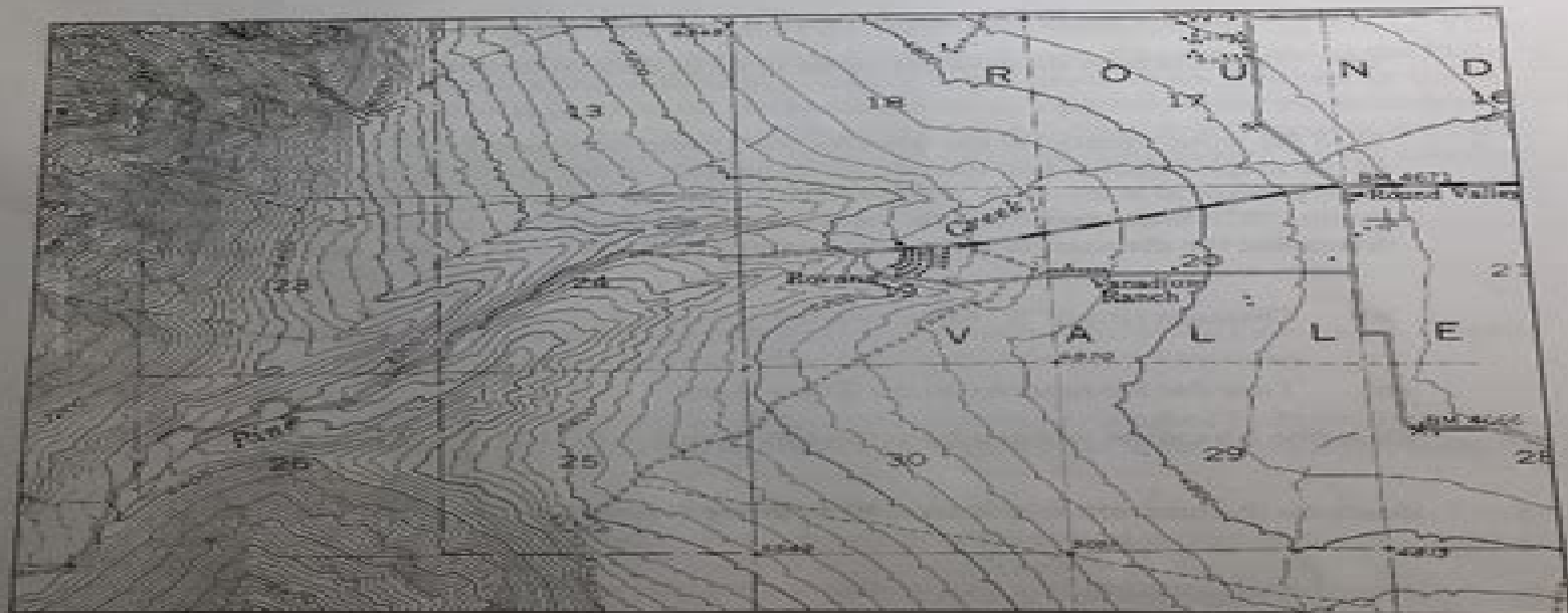
Figure 48-8: USGS "Mt. Tom, California" quadrangle (enlarged to scale 1:48,000; contour interval 80 feet; ↑N).
