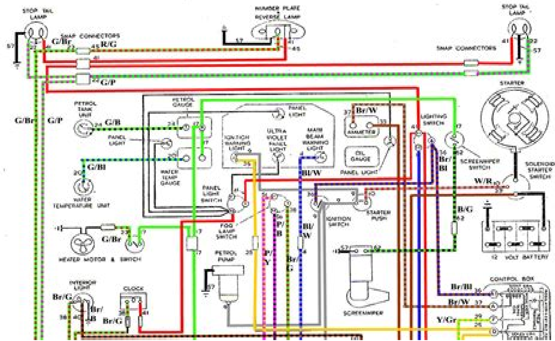
WIRING DIAGRAM—R.H.D. (Commencing Car No. ZB18577)
