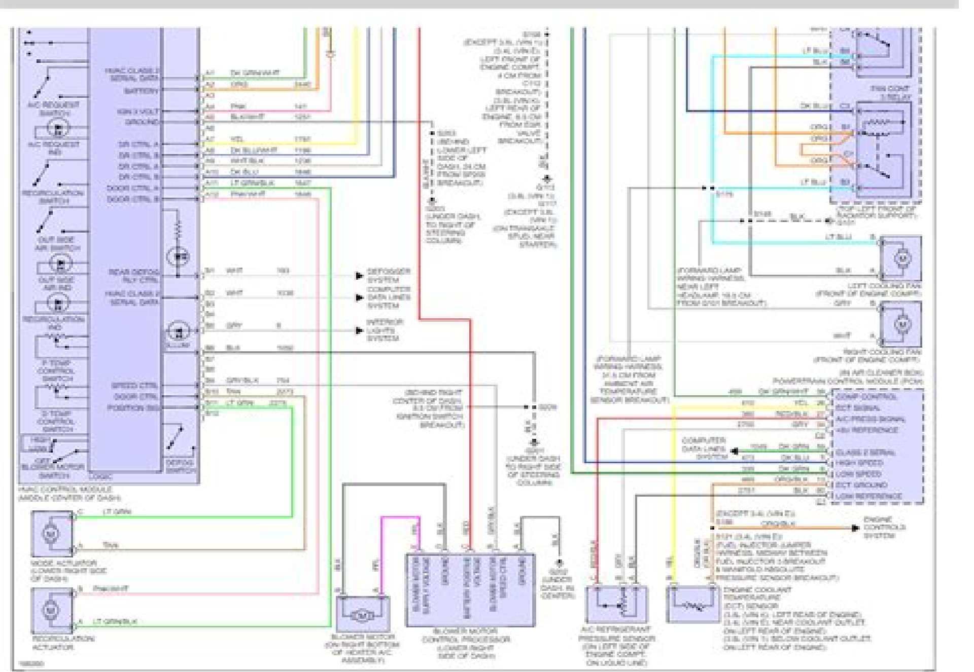
Fig 2: Manual A/C Circuit
