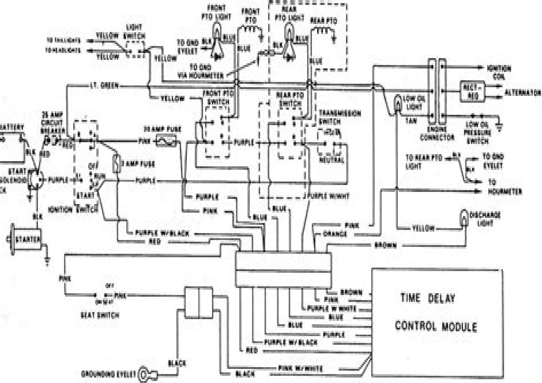
Fig. JD18—Wiring diagram for Model 316 serial number 70,001-285,000 and 318 and 420 models prior to 475,000.
