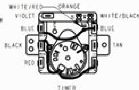
WIRING DIAGRAM - GAS
