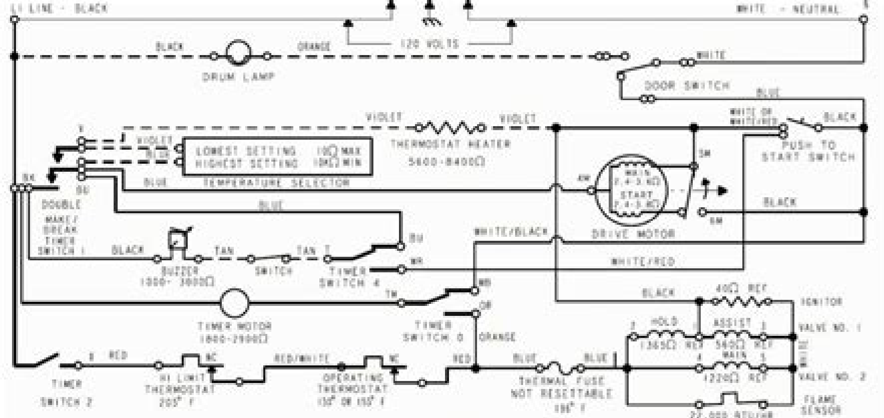
WIRING DIAGRAM - GAS
