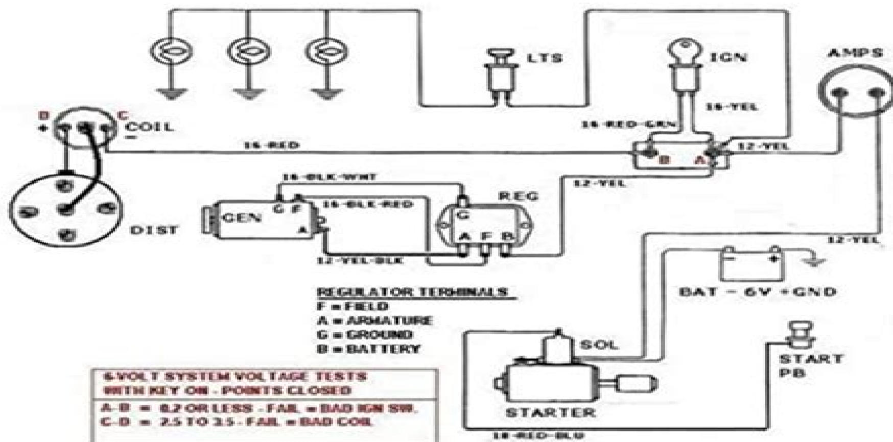
FORD 8N TRACTOR WIRING - SIDE DISTRIBUTOR 1950 TO 1953 Jubilee K.LaRue - Free of Charge - 2006
