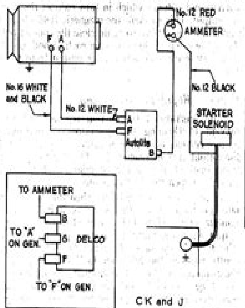
GENERATOR CIRCUIT
