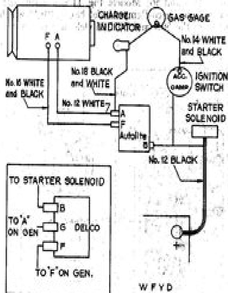
GENERATOR CIRCUIT
