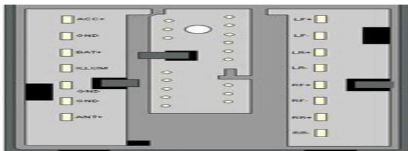
15 pin Ford Car Stereo proprietary connector
