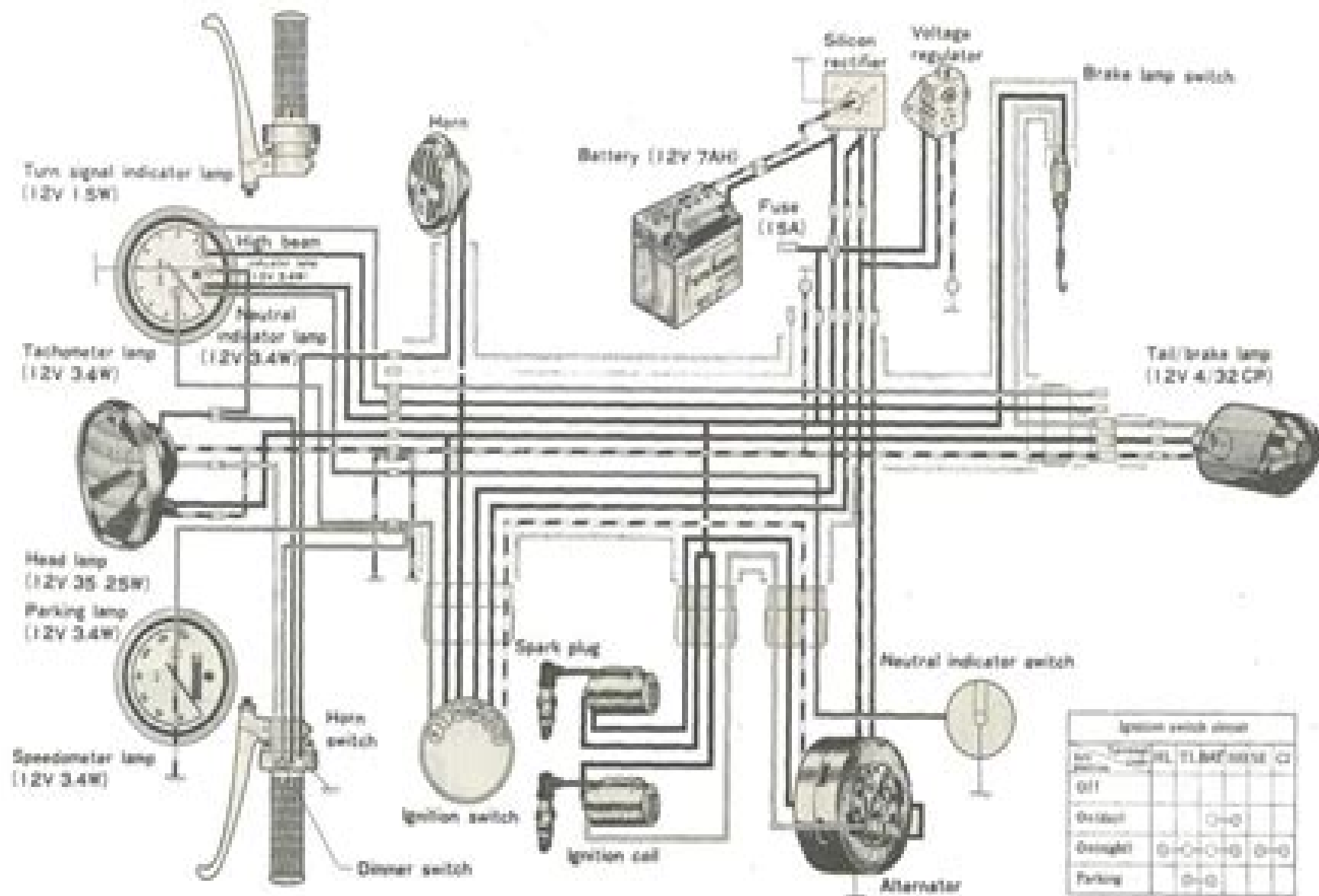
Suzuki T500 wiring diagram.
