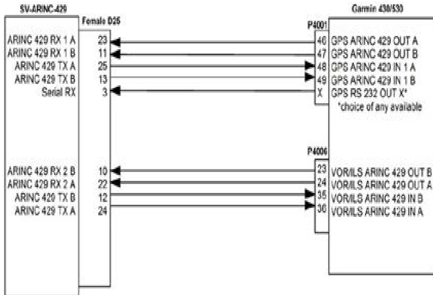
Figure 182 – Garmin 430/530 SV-ARINC-429 Connections
