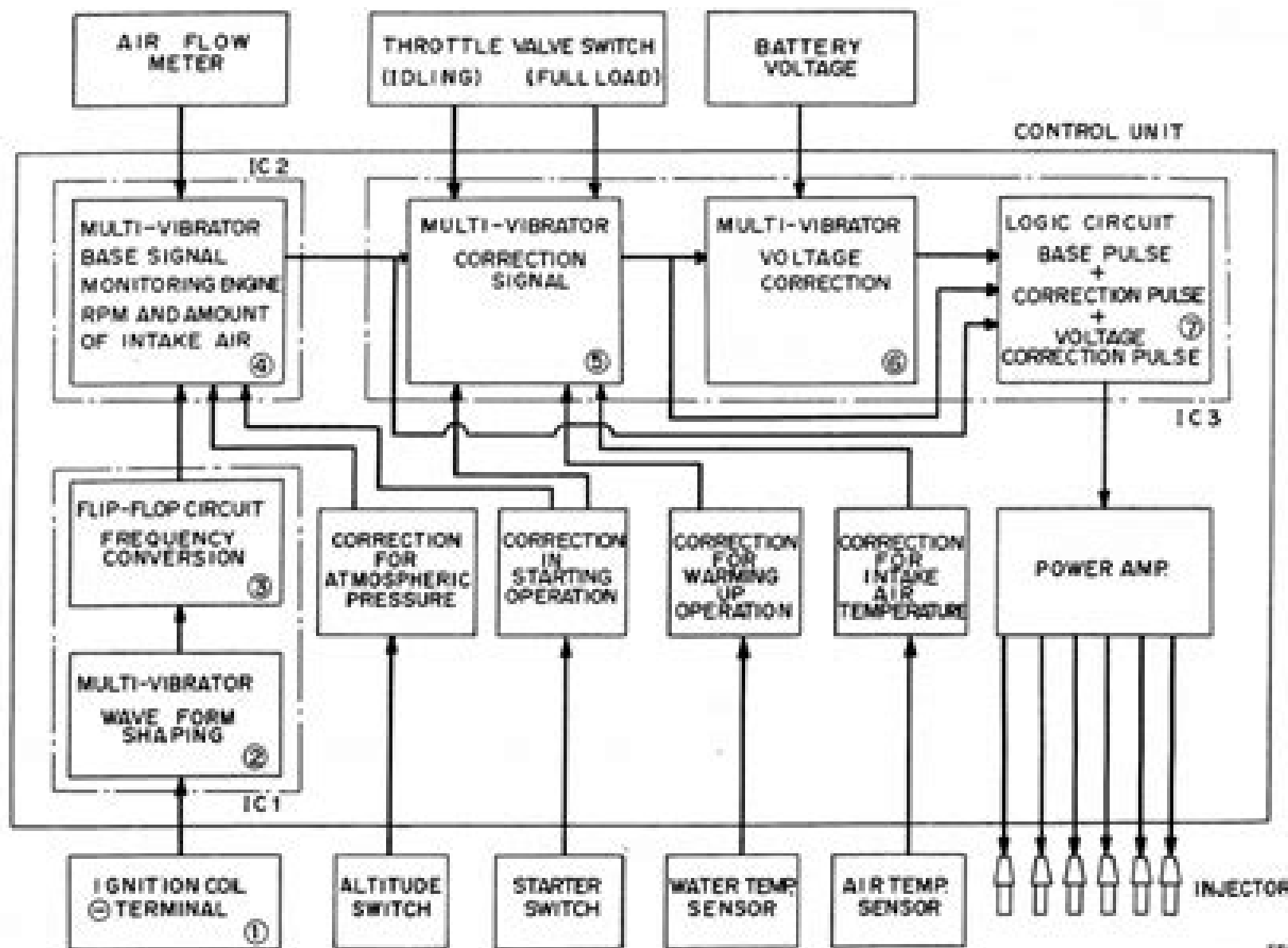
Fig. EF-4 Control unit block diagram
