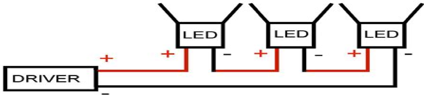
SERIES WIRING CONSTANT CURRENT
