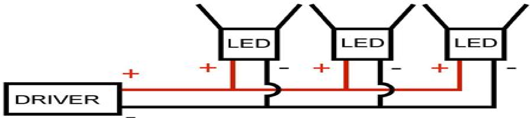
PARALLEL WIRING CONSTANT VOLTAGE
